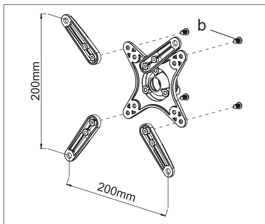
For VESA 200x200
