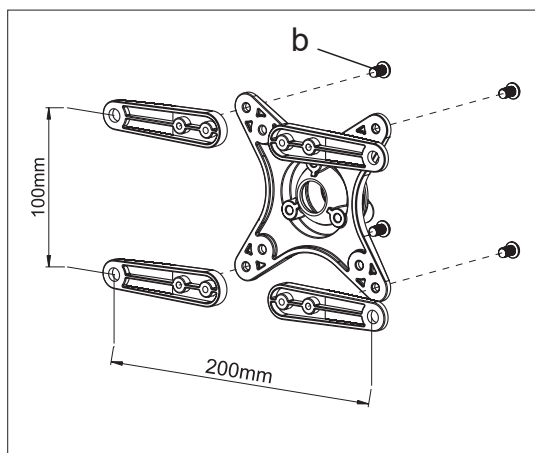
For VESA 200x100
